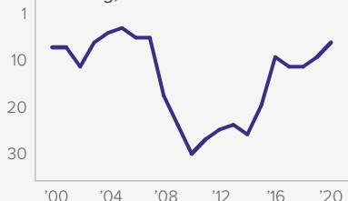
Ranking, 2000–2020 ▲ 1
