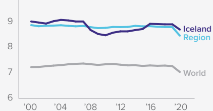
Score, 2000–2020 ▼ 0.31
